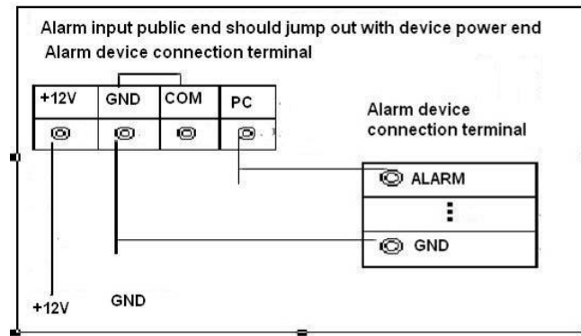
Figure 4-3 Alarm input
