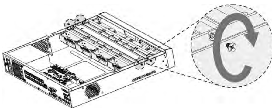
Figure 2-21 Fasten screws
