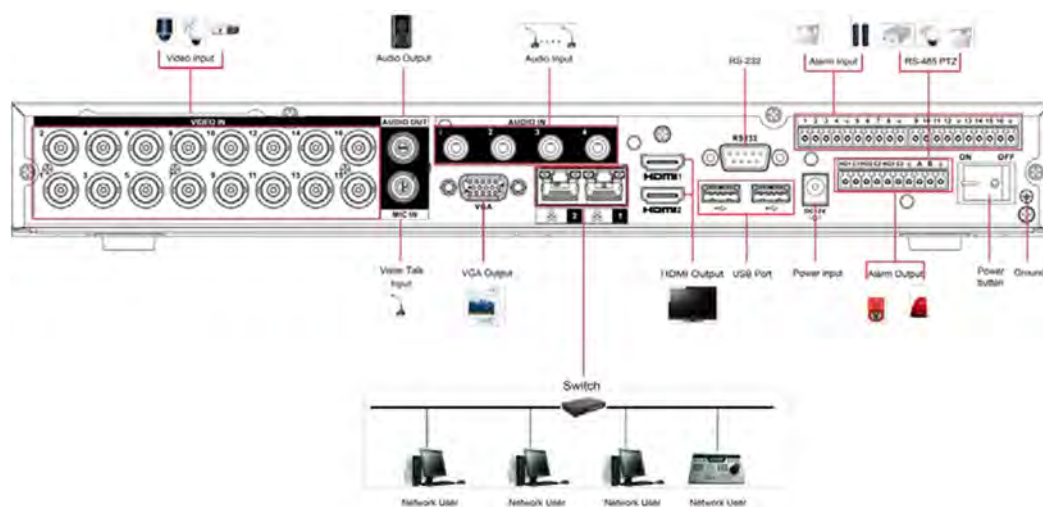
Figure 4-1 Connection diagram
