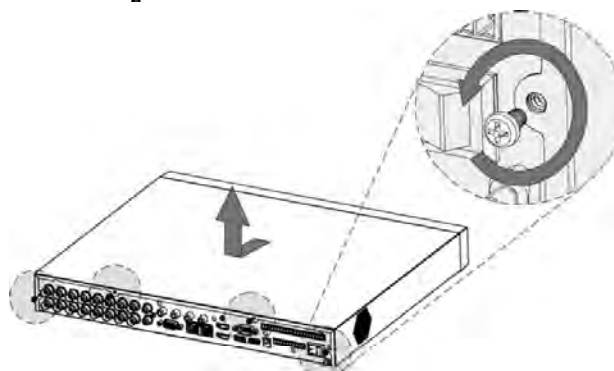
Figure 2-1 Remove screws
