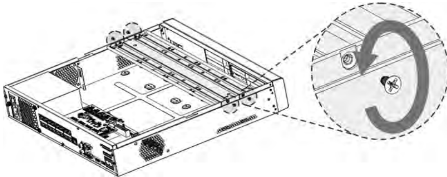
Figure 2-18 Remove bracket
