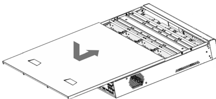
Figure 2-23 Put backcover
