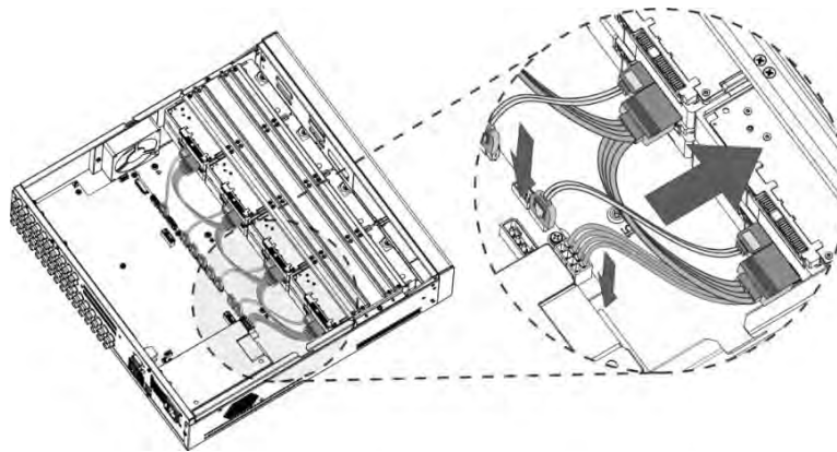
Figure 2-14 Connect cables
