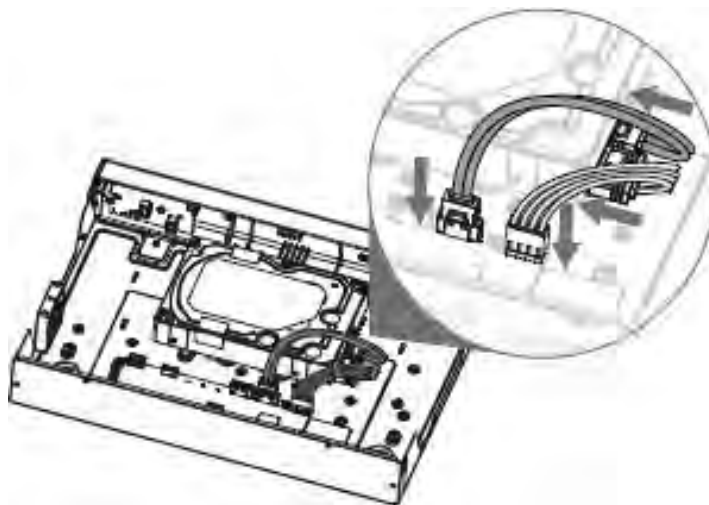
Figure 2-27 Connect cables
