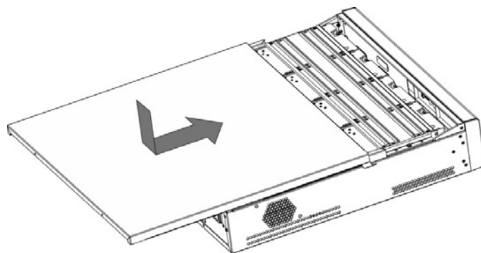
Figure 2-15 Put backcover
