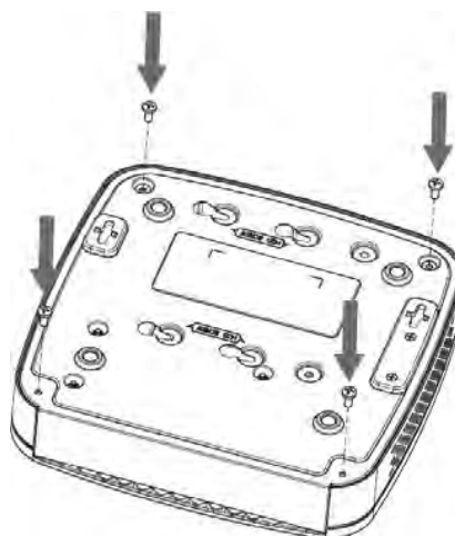
Figure 2-35 Fasten screws
