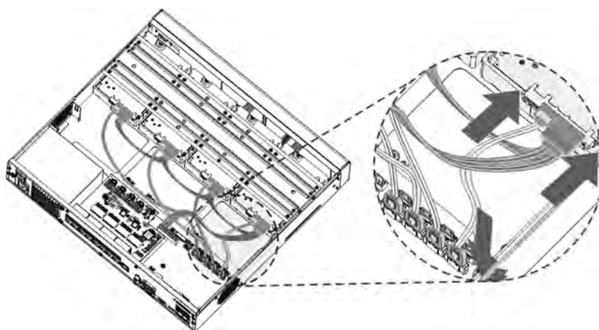
Figure 2-22 Connect cables
