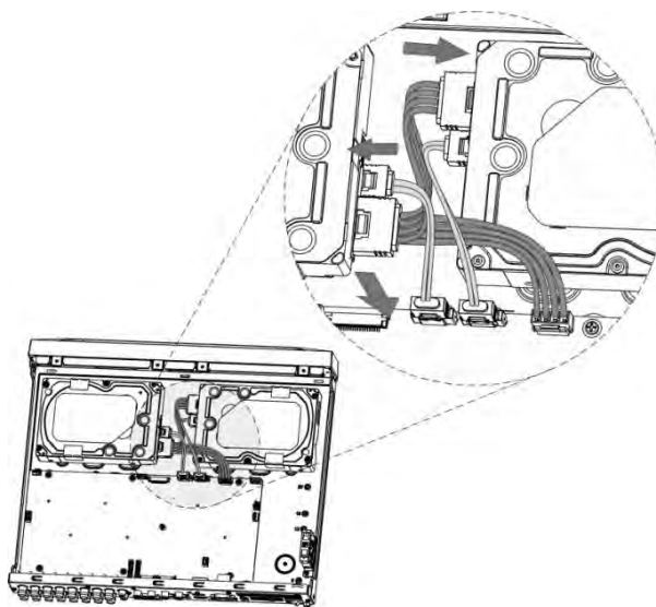
Figure 2-5 Connect cables
