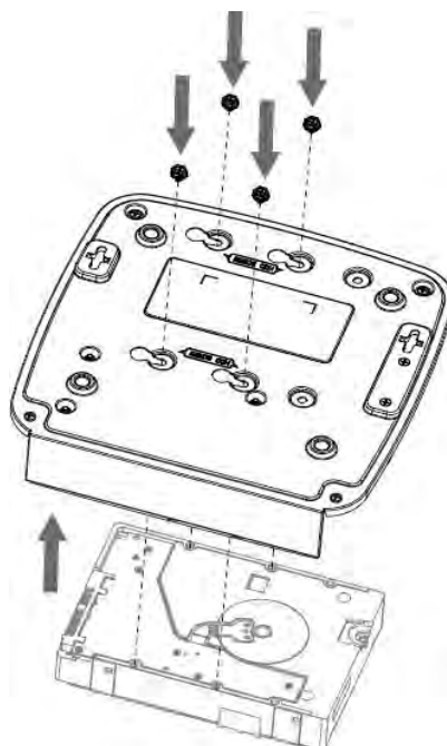
Figure 2-32 Install HDD
